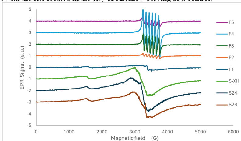
Fig. EPR spectra of samples from a single site: F1 – needle from litter, F2 – young needle, F3 – secondary needle, F4 – tertiary needle, F5 – oldest needle, S-XII – litter, S24 – topsoil, and S26 – soil from a depth of 5 cm.
