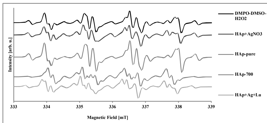
Figure 1. Summarizes the EPR spectra of all samples of hydroxyapatite and spin trap DMPO with the solvent DMSO with \text{H}_2\text{O}_2 without irradiation.
